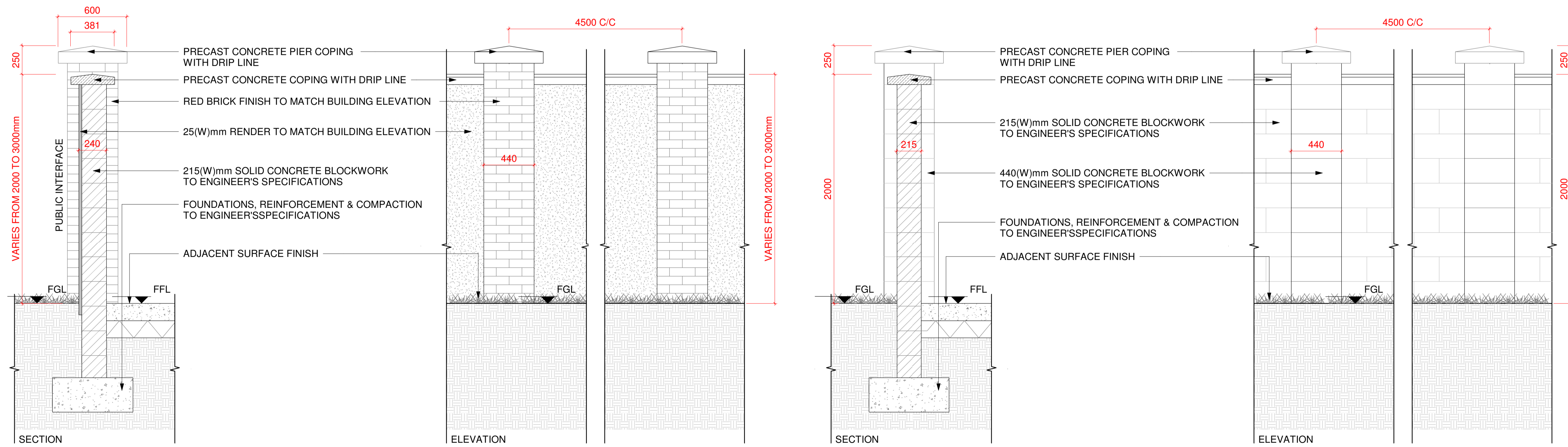
7 TYPICAL DETAIL: 2m HIGH BLOCK WALL SCALE: 1:20 @A1
