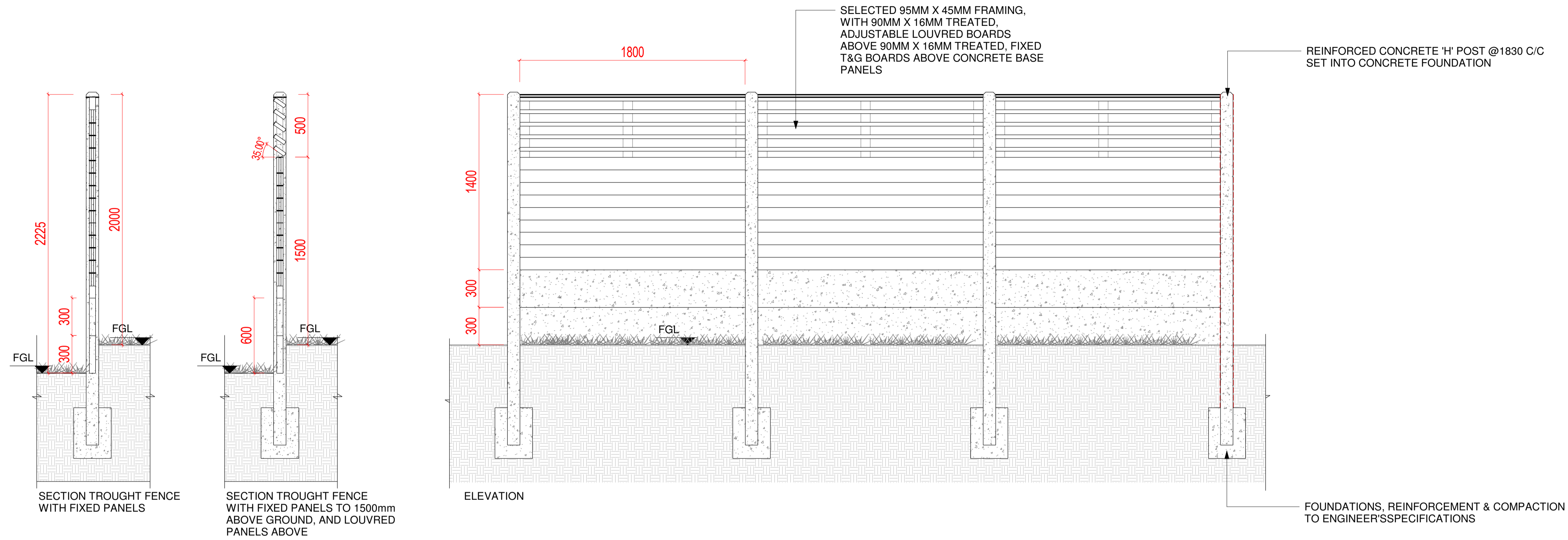
5 TYPICAL DETAIL: 2m HIGH CONCRETE POST & TIMBER PANEL INFILL WITH LOUVRED TOP FENCE SCALE: 1:20 @A1
